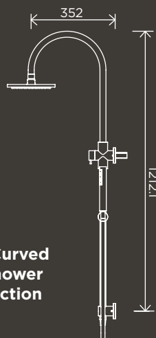
300mm Rose, Curved Combination Shower Rail, Single-Function Hand Shower
