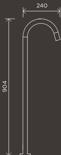
Round Freestanding Bath Spout
