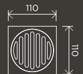
Square Floor Grate Shower Drain 100mm Outlet
