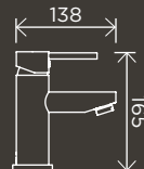
Round Basin Mixer Curved
