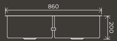
Kitchen Sink - Double Bowl 860 x 440
