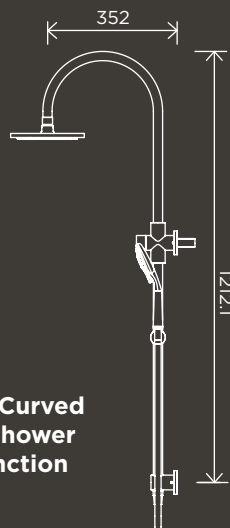
300mm Rose, Curved Combination Shower Rail, Three-Function Hand Shower
