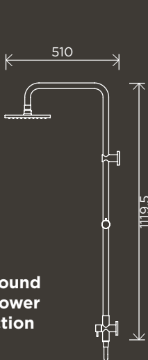
200mm Rose, Curved Combination Shower Rail, Three-Function Hand Shower
