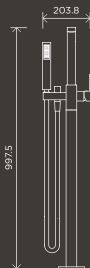
Square Freestanding Bath Spout and Hand Shower
