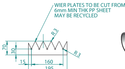
WEIR PLATE 2 REQD PER PIT
