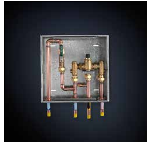
Special 42154 box with bypass, pipes one end (shown without lid).
